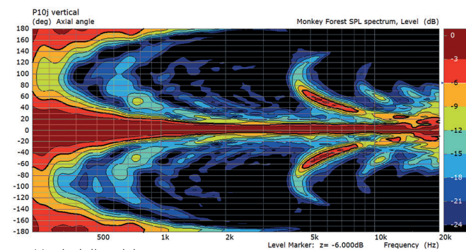
Vertical directivity
