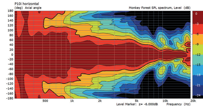
Horizontal directivity
