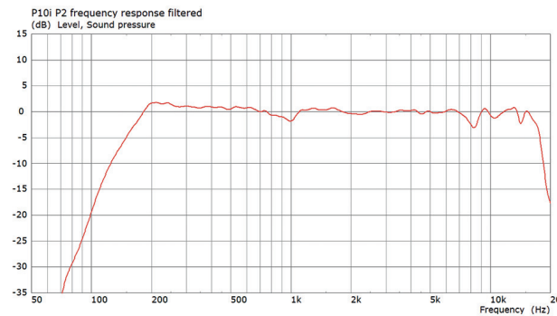
Frequenzgang (processed)
