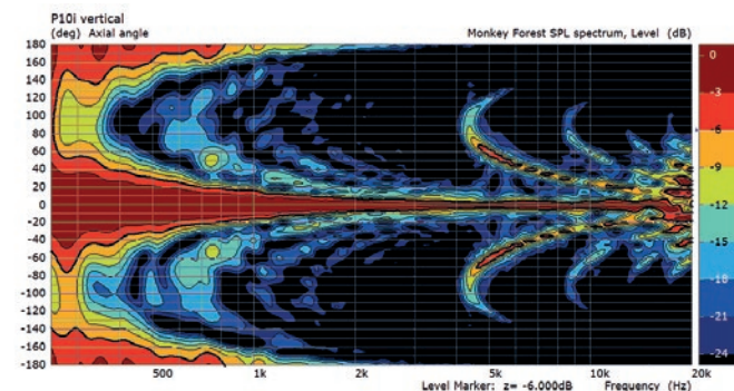
Vertical directivity
